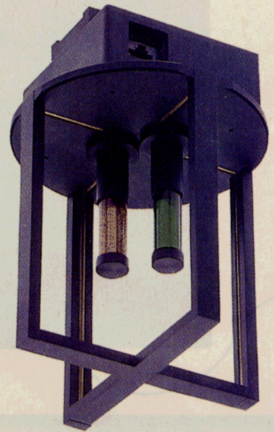
RADIO TRANSCIVER links pads and other movable computer devices to the wired network. This unit, intended to be mounted on the ceiling, contains antennas in its crossed arms and two light-emitting diodes to signal its status.
