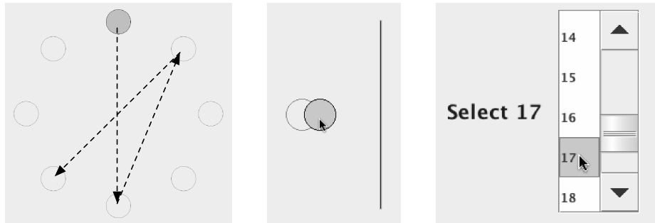
Fig. 5. SUPPLE’s pointing, dragging, and list selection tasks from the ability-assessment battery. From these tasks, SUPPLE builds a predictive model of a user’s movement time that is used to parameterize a search for the “optimal” interface. Widget selection, size, position, and grouping are all part of the search space.
